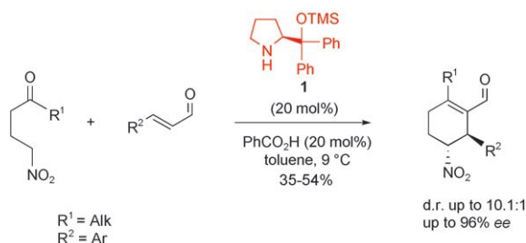
Scheme 7. Domino reaction of \gamma -nitroketones and enals.
