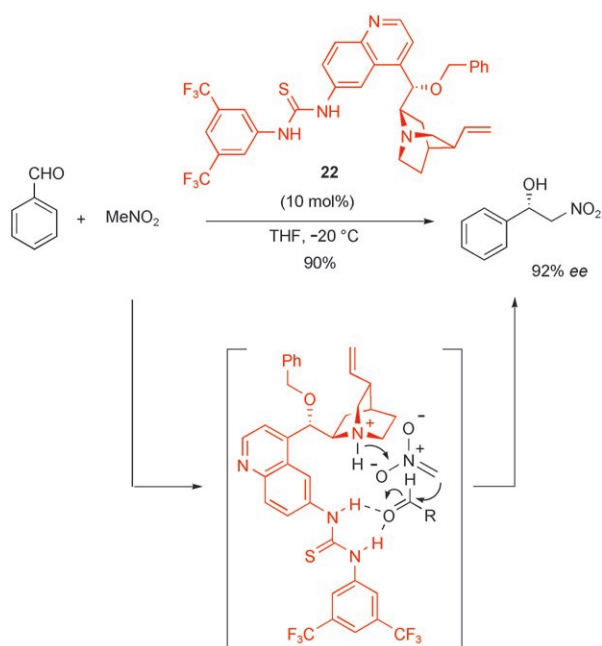
Scheme 23. Asymmetric organocatalytic Henry reaction with electro-ophile/nucleophile activation.
