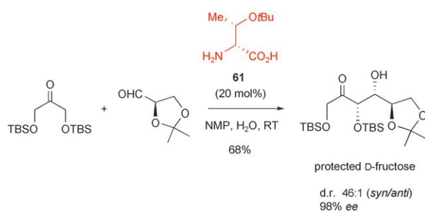
Scheme 40. Synthesis of protected D-fructose. NMP = N -methyl-2-pyrrolidinone.
