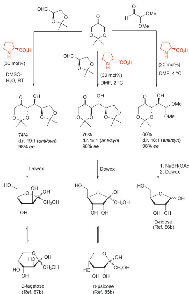
Scheme 39. The biomimetic C_3 + C_n strategy for the synthesis of carbohydrates.
