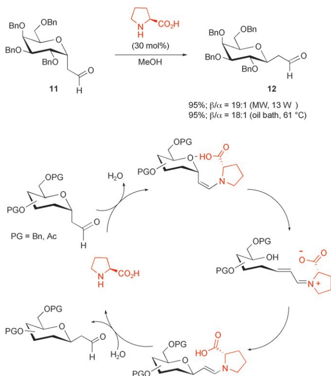
Scheme 15. Microwave-assisted organocatalytic anomerization of \alpha -C-glycosylmethyl aldehydes. PG = protecting group, Bn = benzyl.
