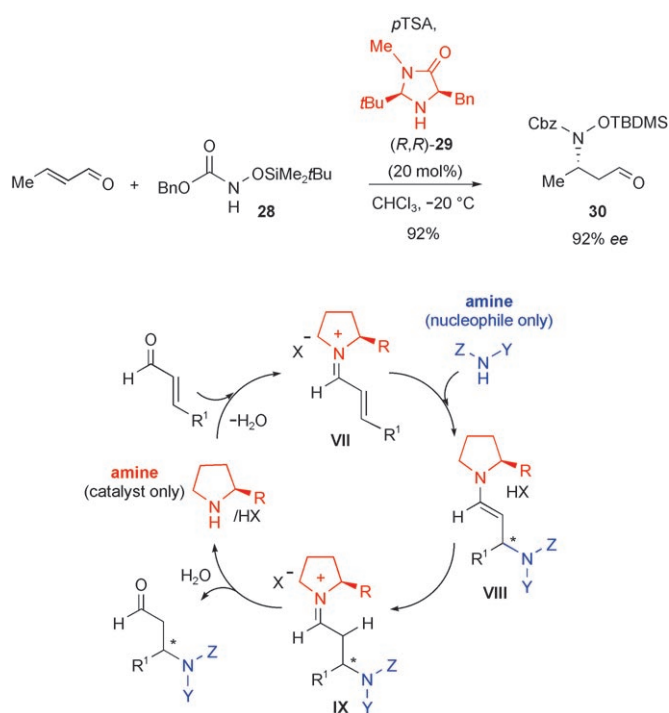
Scheme 26. Enantioselective organocatalytic conjugate addition of an amine. Cbz = benzyloxycarbonyl, TBDMS = tert -butyldimethylsilyl.
