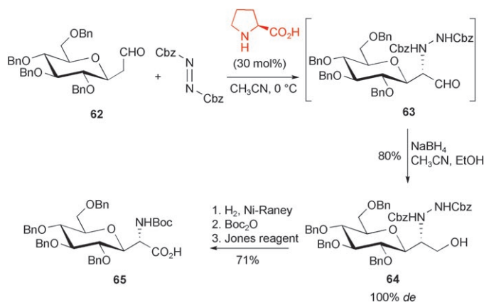
Scheme 41. Organocatalytic synthesis of C -glycosylglycines. CBz = benzyloxycarbonyl.
