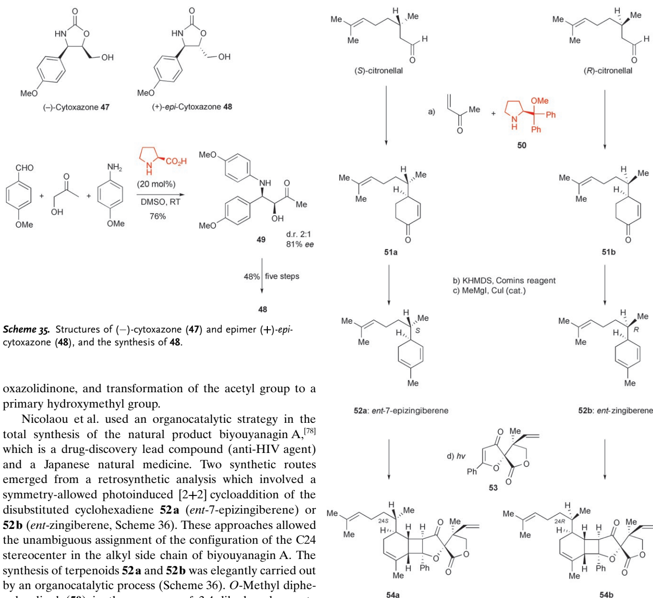
Scheme 36. Total synthesis of biyouyanagin A ( 54b ). HMDS = 1,1,1,3,3,3-hexamethyldisilazane.
