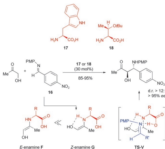
Scheme 20. Organocatalytic asymmetric synthesis of anti -1,2-amino alcohols.
